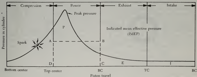
FIGURE 1-28. Cylinder pressure during power cycle.
